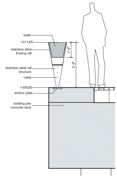
SECTION B-B FLOWING RAIL
